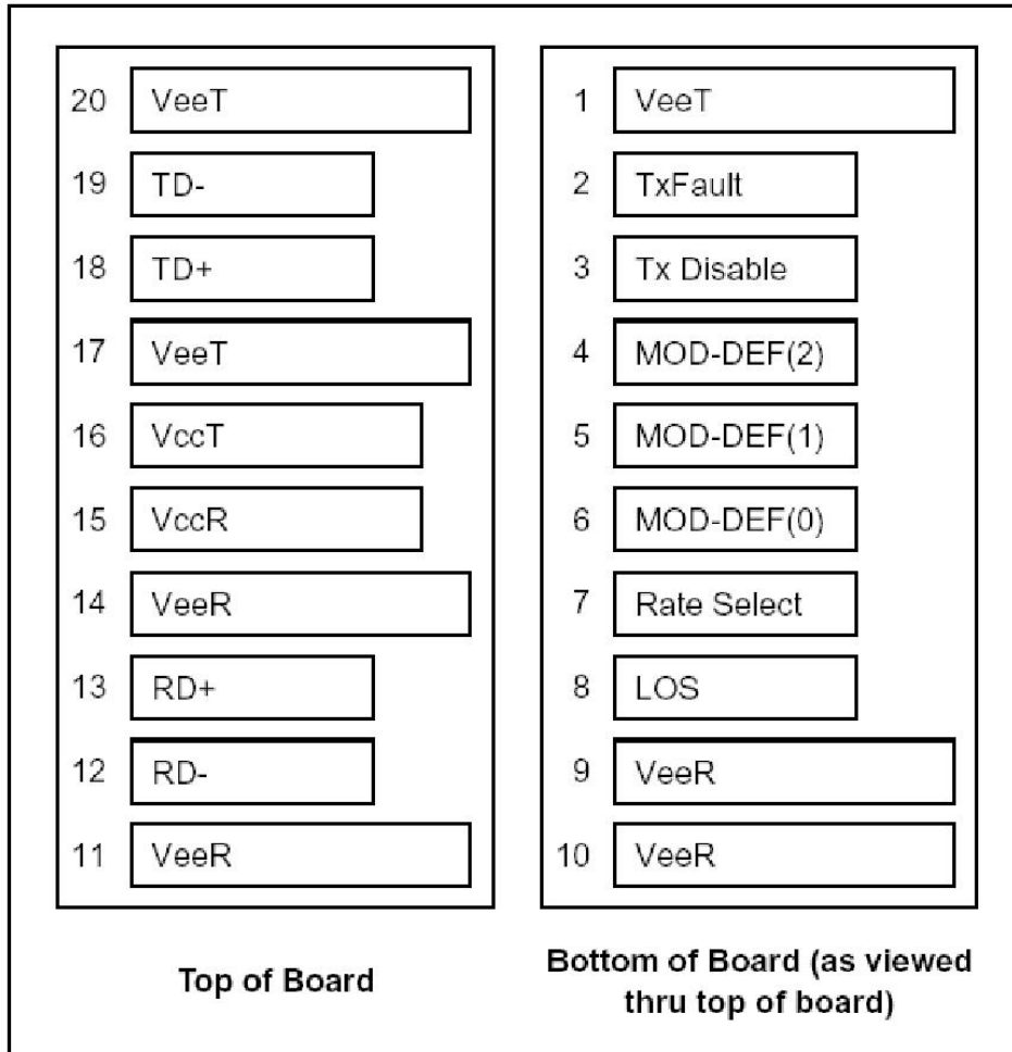
Figure 1. Pin Definitions
